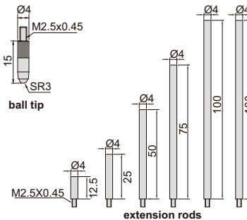
extension rods
