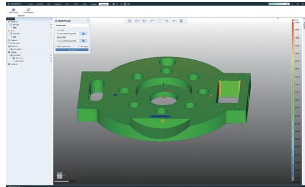
deviation analysis
